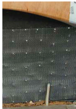
FIG.1A-ATTACHING LATH, FIG.1B-APPLYING SCRATCH COAT OF MORTAR
